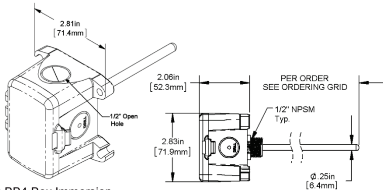
Figure 2: BB4 Box Immersion Part #s NSB-10K-2-I-2-BB4 (2" probe, no thermowell) NSB-10K-2-I-4-BB4 (4" probe, no thermowell) A Pierceable Knockout Plug (Part # NSB-PKP-100) is available for the open port in the BB4
