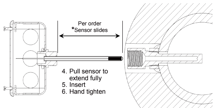
Figure 13: Standard J-Box Before Insertion
