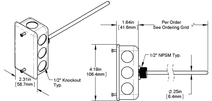
Figure 3: J-Box Immersion (Standard) Part #s NSB-10K-2-I-2 (2" probe, no thermowell) NSB-10K-2-I-4 (4" probe, no thermowell) NSB-10K-2-I-2-M304 (2" probe, 304 SS thermowell) NSB-10K-2-I-4-M304 (4" probe, 304 SS thermowell)
