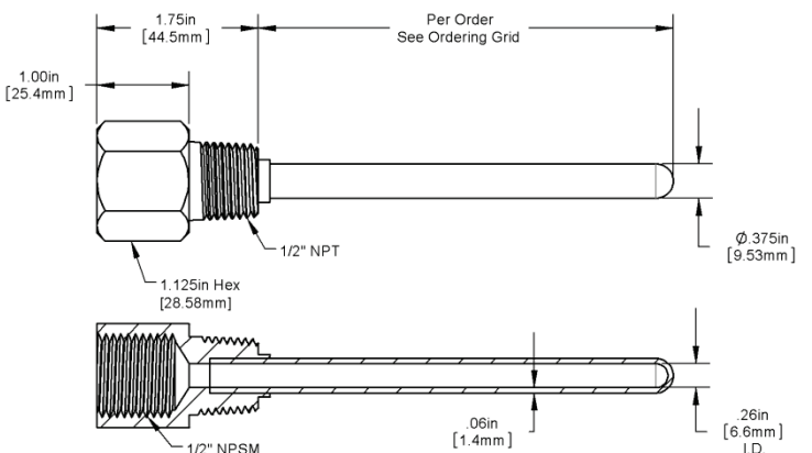
Figure 5: Two-Part Welded Thermowell
