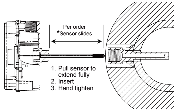
Figure 11: BB4 Sensor Before Insertion
