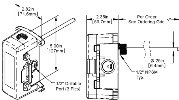
Figure 1: BB2 Box Immersion Part #s NSB-10K-2-I-2-BB2 (2" probe, no thermowell) NSB-10K-2-I-4-BB2 (4" probe, no thermowell) NSB-10K-2-I-2-M304 (2" probe, 304 SS thermowell) NSB-10K-2-I-4-M304 (4" probe, 304 SS thermowell)
