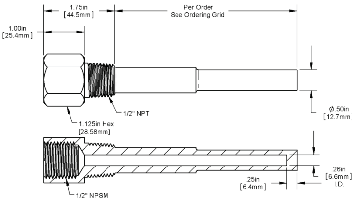
Figure 4: Machined Bar Stock ThermoWell
