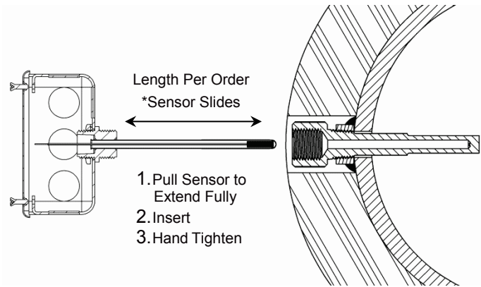
Figure 9: Immersion Sensor Before Insertion
