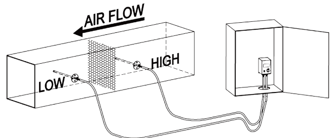
Figure 12: Air filter pressure drop monitoring with the pressure sensor mounted in a panel with two static pressure probes (p/n NSB-ZPS-ACC07) in the duct.
