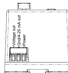
Figure 7: Wiring terminations
