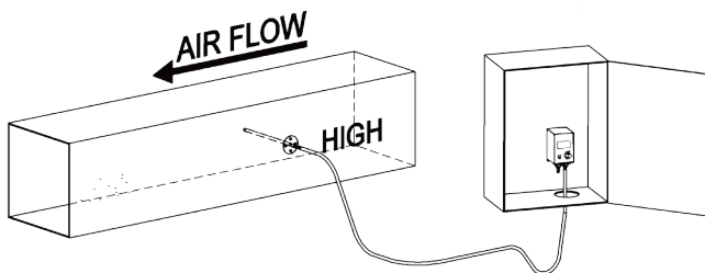
Figure 11: Duct static pressure monitoring with the pressure sensor mounted in a panel with a static probe (p/n NSB-ZPS-ACC07) in the duct.
