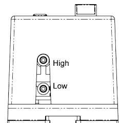
Figure 6: Pressure Port Connections
