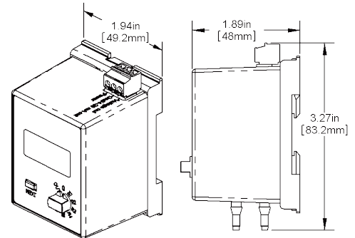
Figure 1: Pressure Sensor
