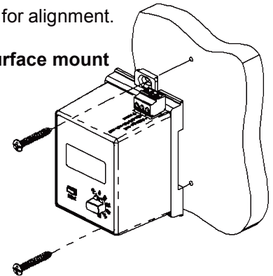
Figure 5: Surface mounting with the tabs out.
