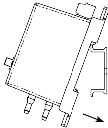
Figure 3: Catch the mounting hook on the edge of the DIN Rail, then rotate into place.
