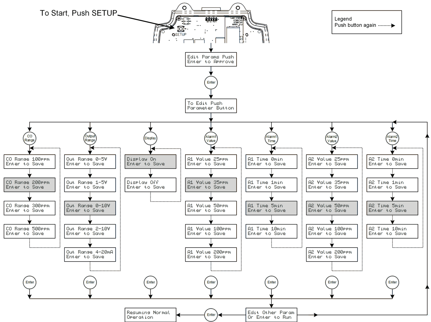
Figure 18: Parameter Setup Flow Chart (Default settings are shown with gray shading)
