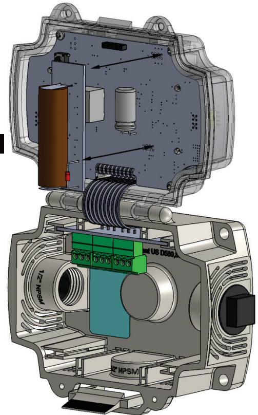
Figure 19: Inserting or Removing the CO Sensor Module
