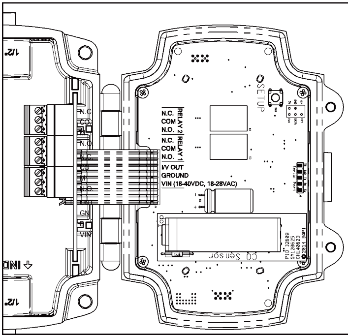
Figure 4: Field Wiring Terminals
