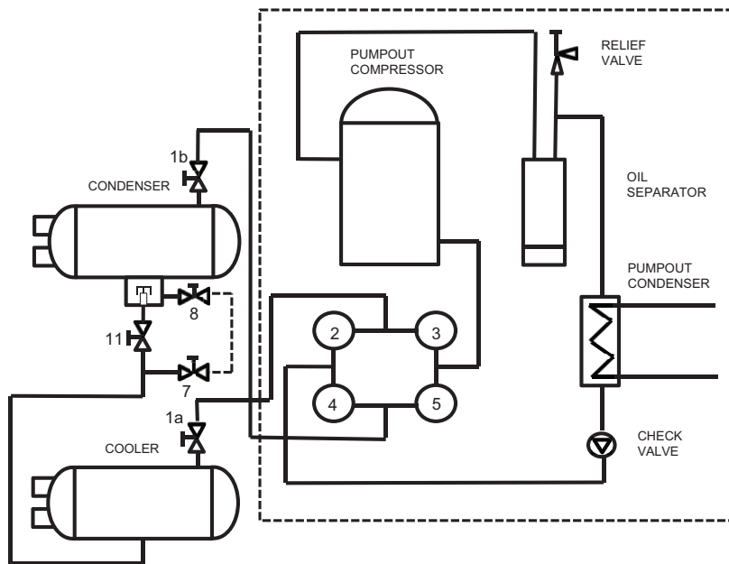
Fig. 11 — Typical Optional Pumpout System Piping Schematic without Storage Tank
