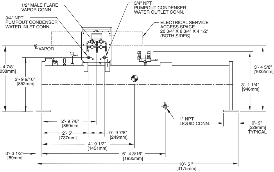
FRONT VIEW
