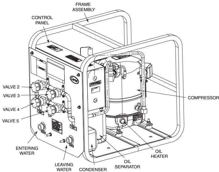
Fig. 9 — Pumpout Unit
