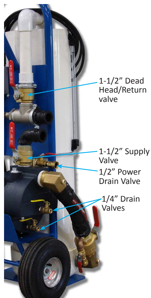
Figure 20: Flush Cart Valves in adding antifreeze steps
