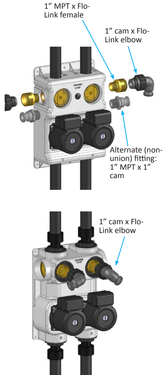
Figure 9: FPT flow center (top) and Flo-Link Double O-ring flow center (below) flush cart fittings
