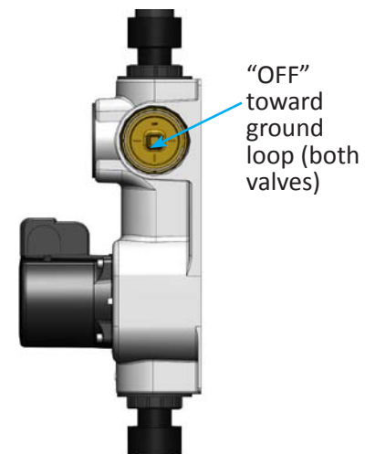
Figure 31: GPM (FPT) flow center (top) and Flo-Link Double O-ring flow center (below) valve positions for ground loop isolation
