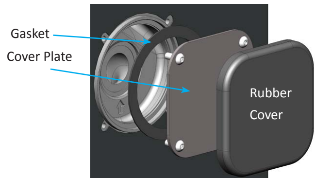
Figure 35: Removing cover plate
