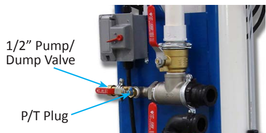
Figure 13: 1/2" Pump & Dump Valve
