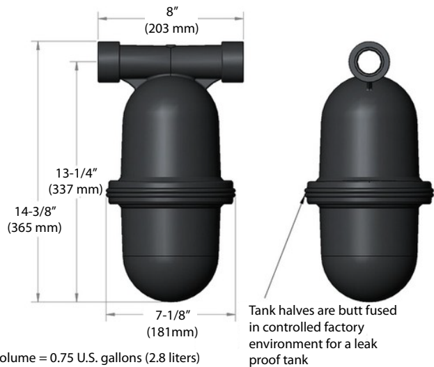
Figure 28: Pressure Battery Expansion Tank
