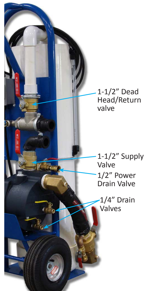
Figure 18: Flush Cart Valves in flushing steps
