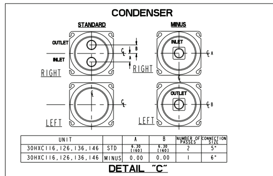
Fig. 3 — Dimensions, 30HXC116-146
