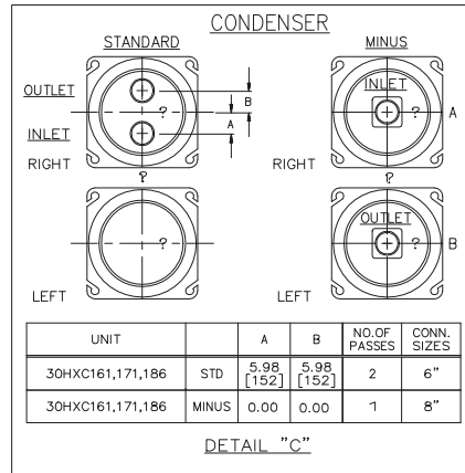
Fig. 4 — Dimensions, 30HXC161-186
