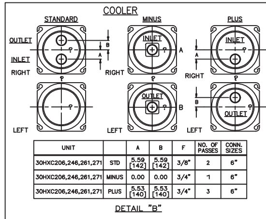
Fig. 5 — Dimensions, 30HXC206-271
