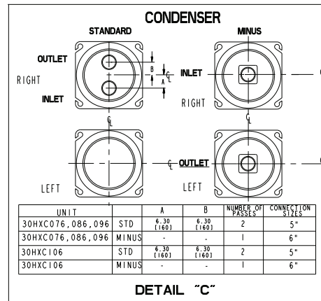
Fig. 2 — Dimensions, 30HXC076-106
