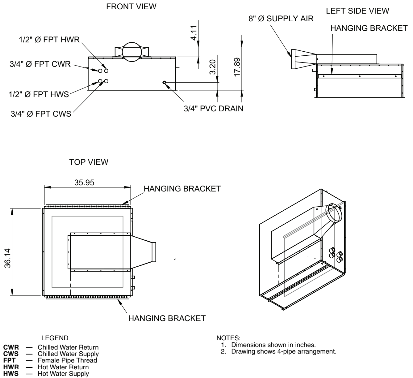
Fig. 4 — 36IBAC 4 x 4, All-Way Blow, 4-Pipe Unit Dimensions
