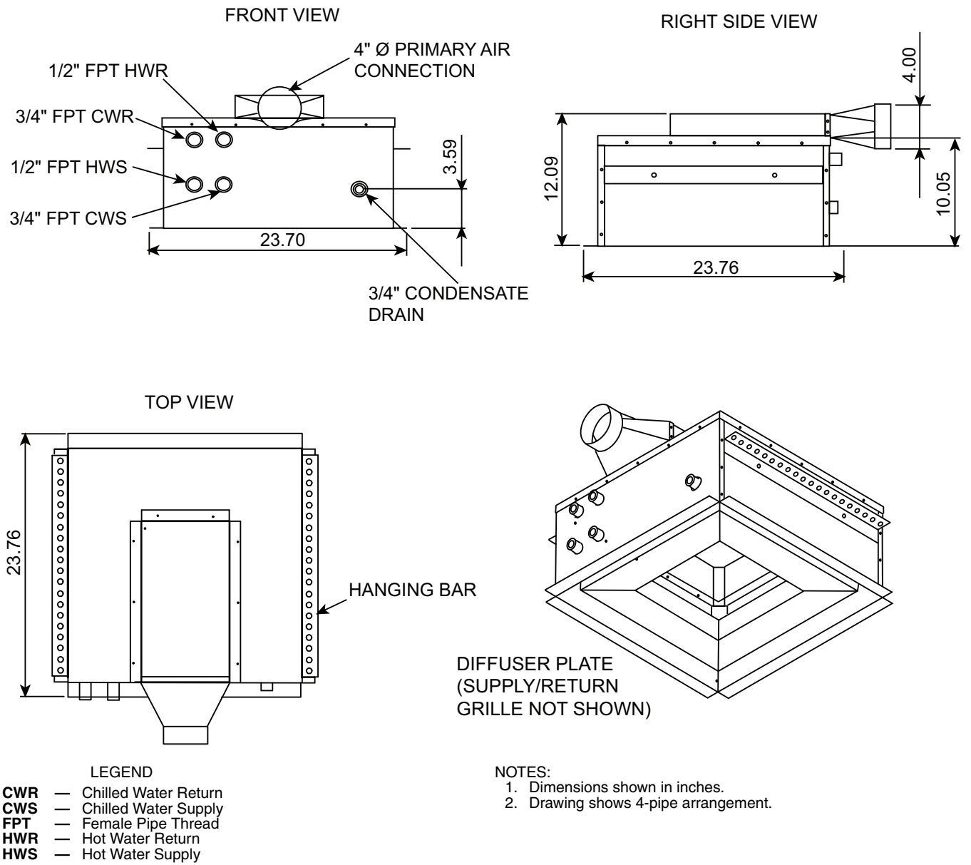
Fig. 2 — 36IBAC 2 x 2, All-Way Blow, 4-Pipe Unit Dimensions
