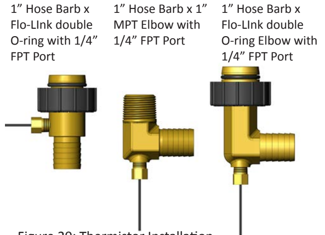
Figure 20: Thermistor Installation
