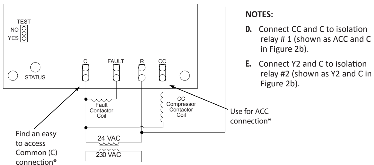
Figure 2c: Wiring Diagram for heat pumps with an external compressor contactor, but without an accessory relay -- see Note A, previous page
