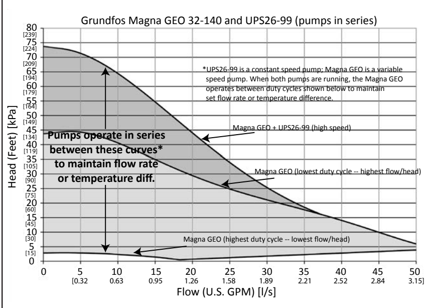
Curves are manufacturer's reported averages using water at 68°F [20°C].
