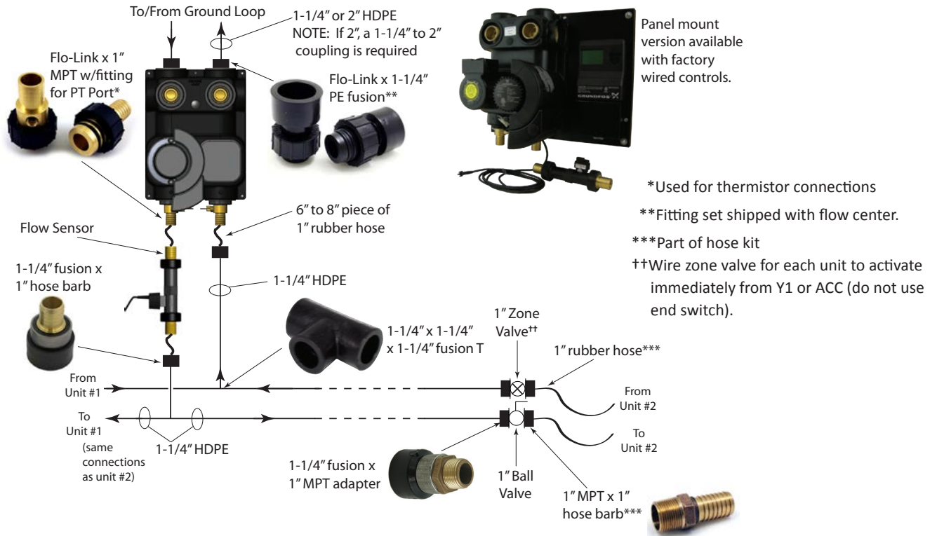
Figure 4a: Two Unit Piping Diagram: Pressurized Flow Center
