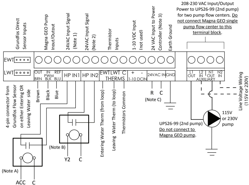
Figure 2b: Wiring Diagram for heat pumps requiring an additional isolation relay -- see Notes A & B, above
