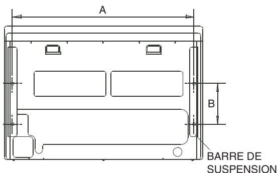
Figure 6 — Emplacements du support de suspension
