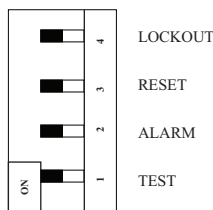
Fig. 18 — Dip Switch Settings
