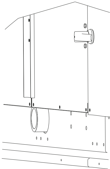
Fig. 32 — Condensate Drain Connection
