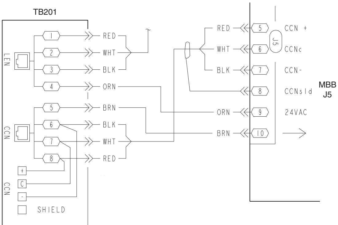
Fig. 83 — CCN Connections
