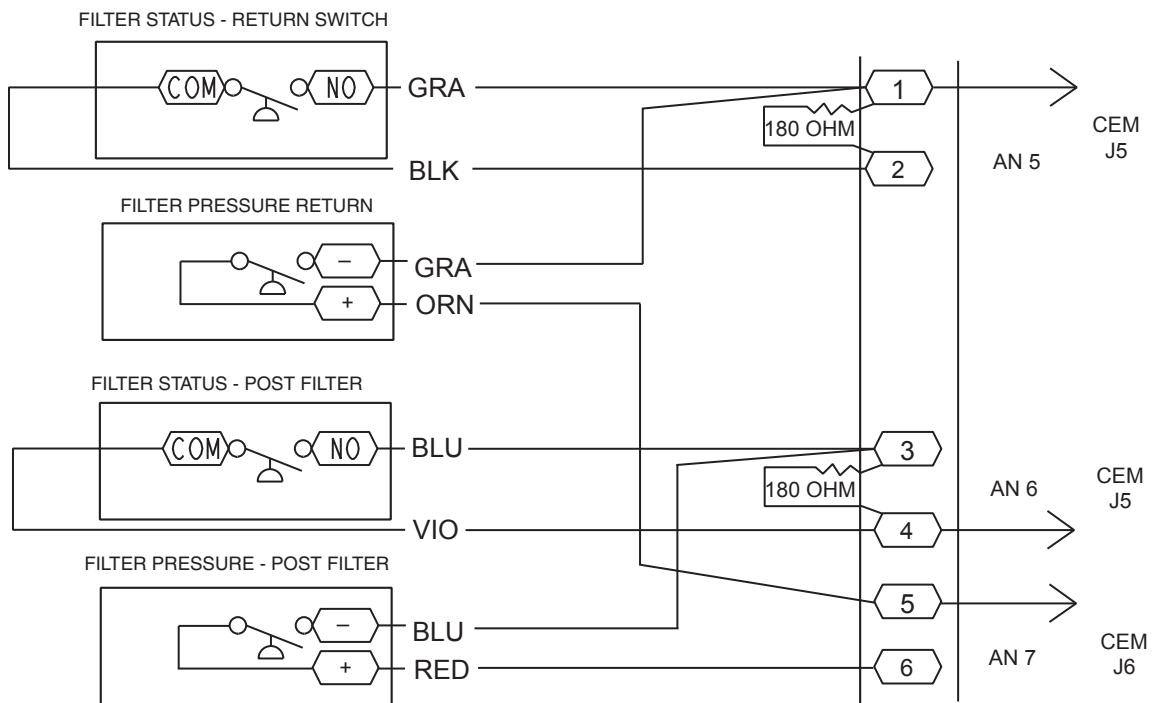
Fig. 76 — Filter Status Wiring
