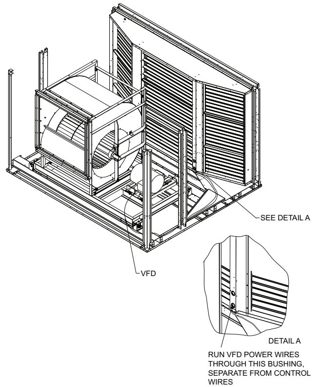
Fig. 67 — Wire Routing
