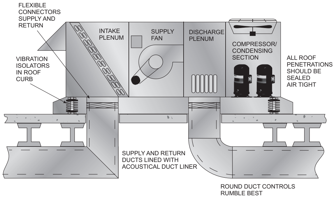
Fig. 1 — Acoustical Considerations
