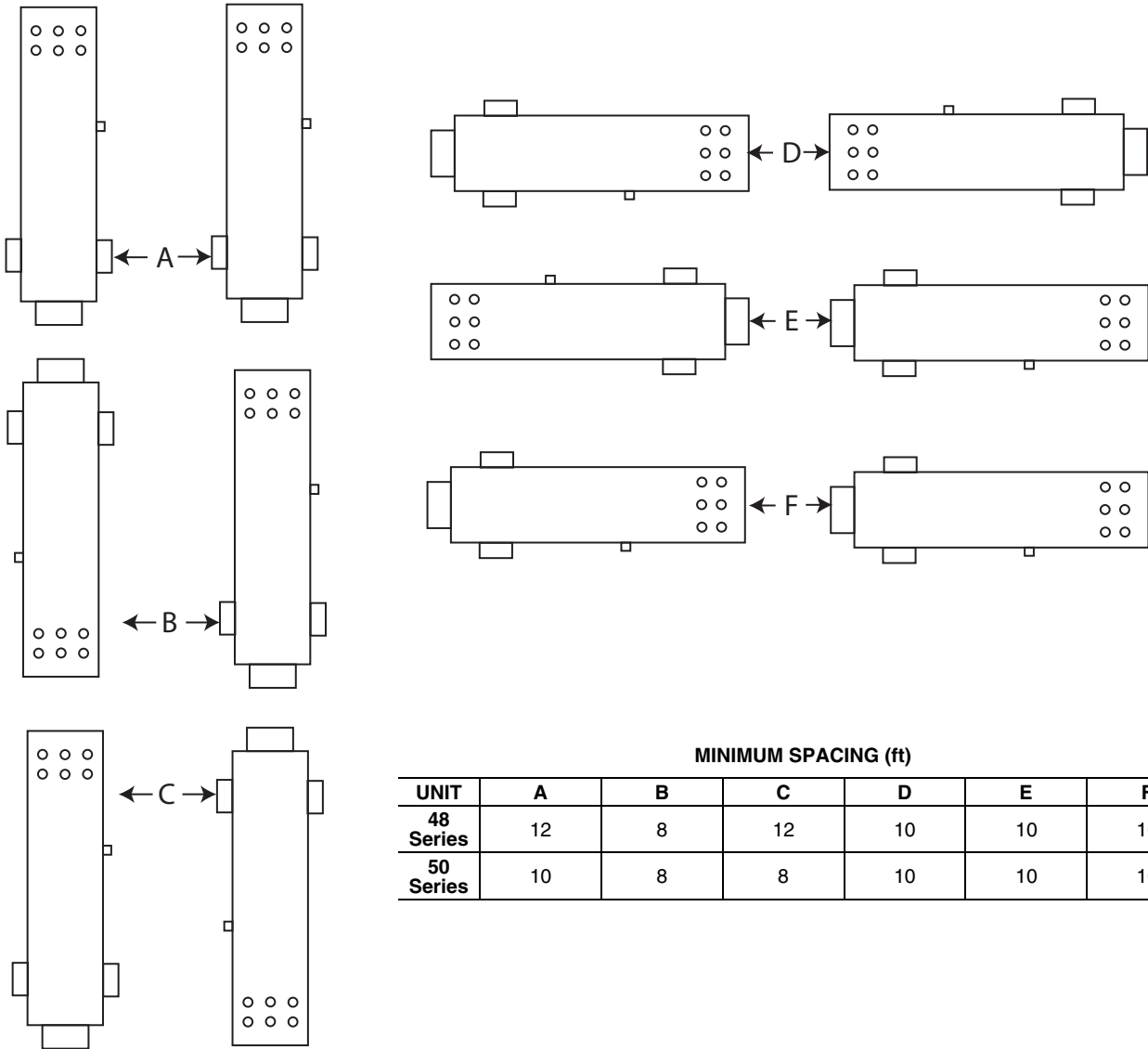
Fig. 2 — Multiple Unit Minimum Separation
