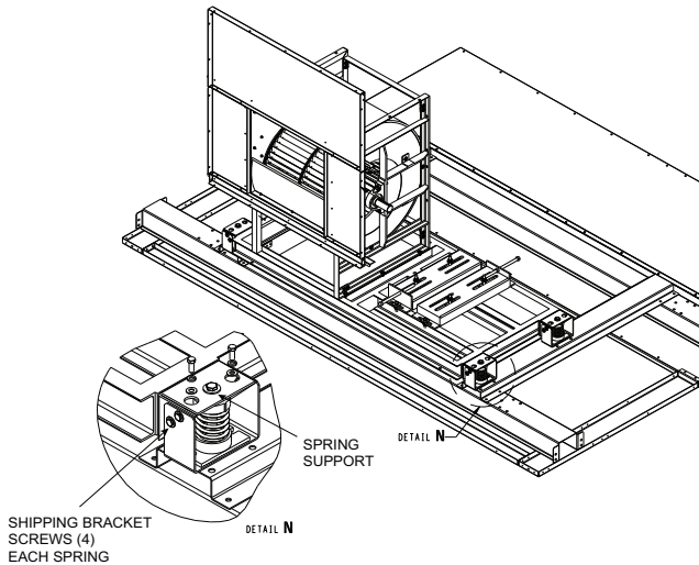
Fig. 49 — Supply Fan and Power Exhaust Fan Shipping Bracket Bolts
