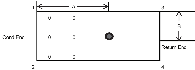
Fig. 29 — Weight Distribution and Center of Gravity
