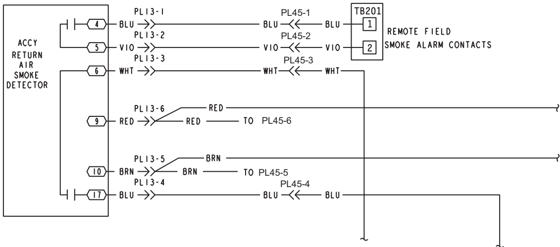
Fig. 80 — Return Air Smoke Detector Wiring
