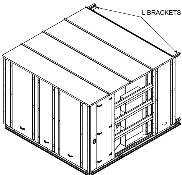
Fig. 60 — L Bracket Removal
