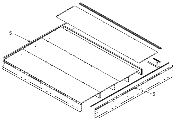
Fig. 24 — Gasket Location — Condenser Section Roof Curb
