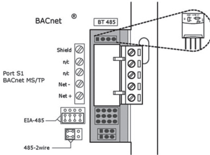
Fig. 86 — BT485 Installation
