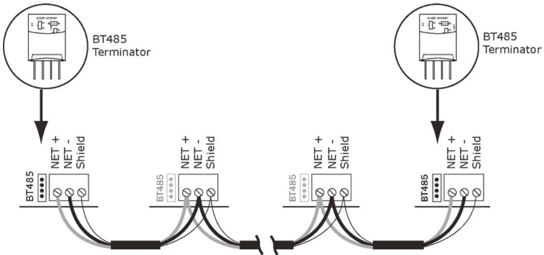
Fig. 85 — Open System Network Wiring
