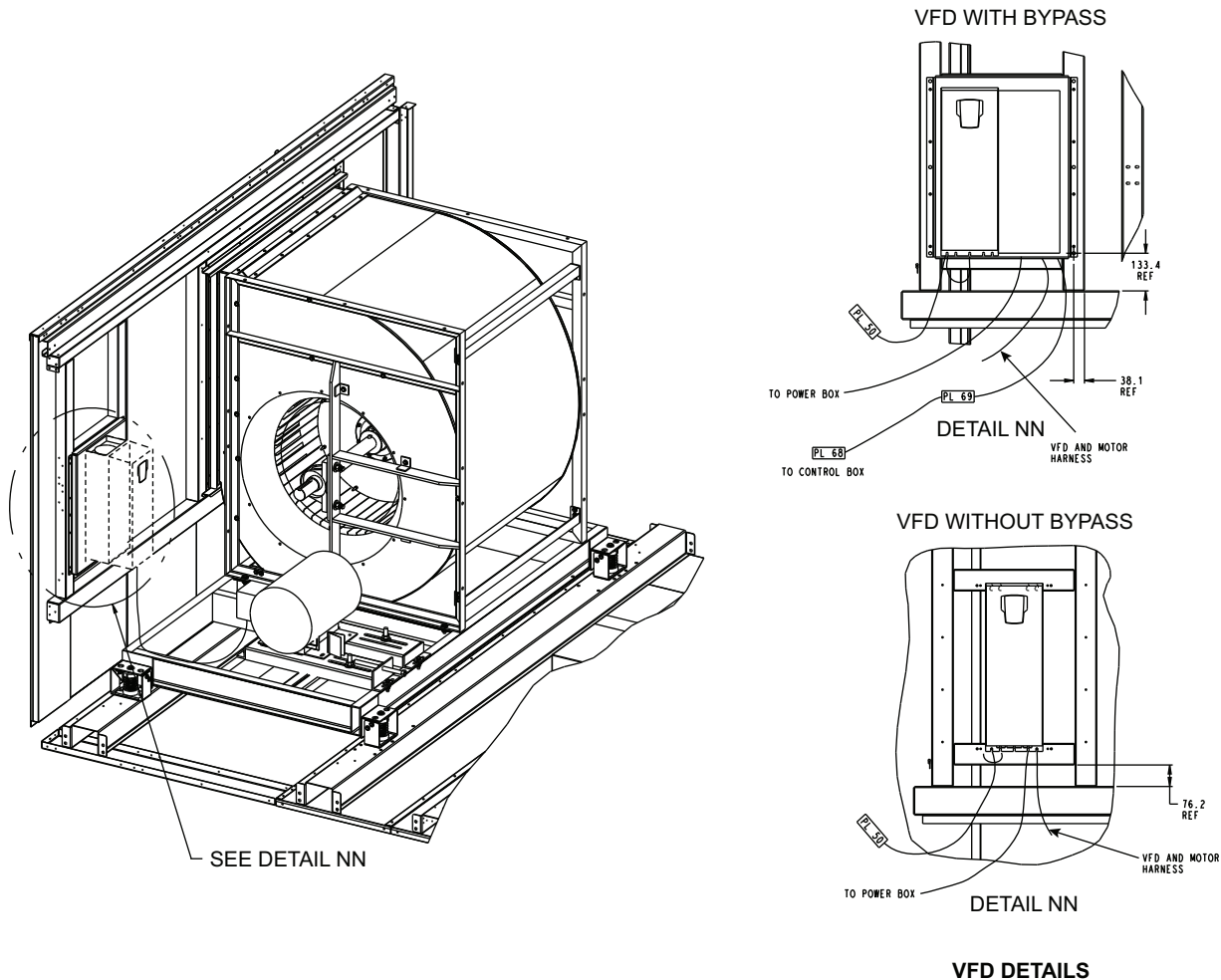
Fig. 68 — Return Section Component Locations
