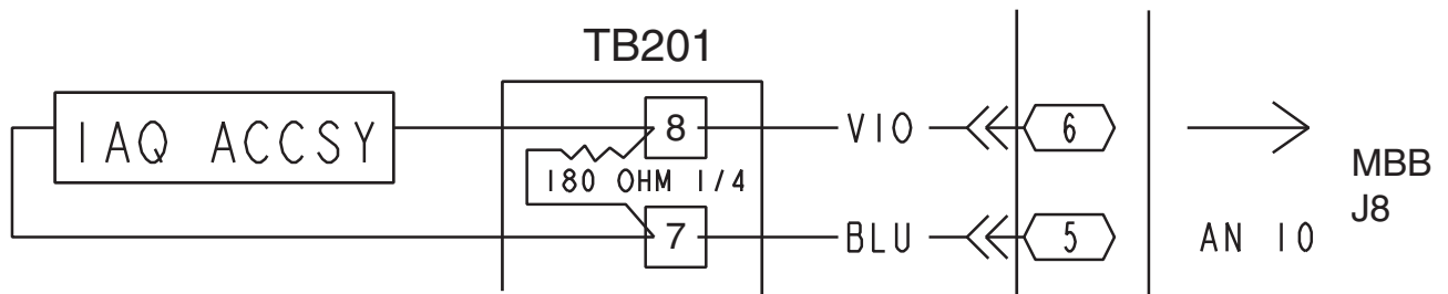
Fig. 75 — CO 2 Space Sensor Wiring
