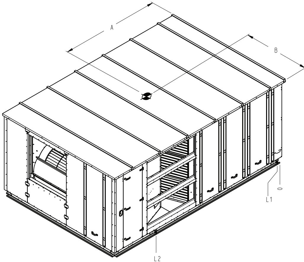
Fig. 27 — 50N 75-150 Ton Split (Return Section) Rigging
