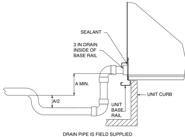
Fig. 33 — Condensate Drain Piping Details (Slab and Curb Mounted)
