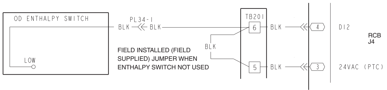
Fig. 74 — Outdoor Air Enthalpy Switch Wiring
