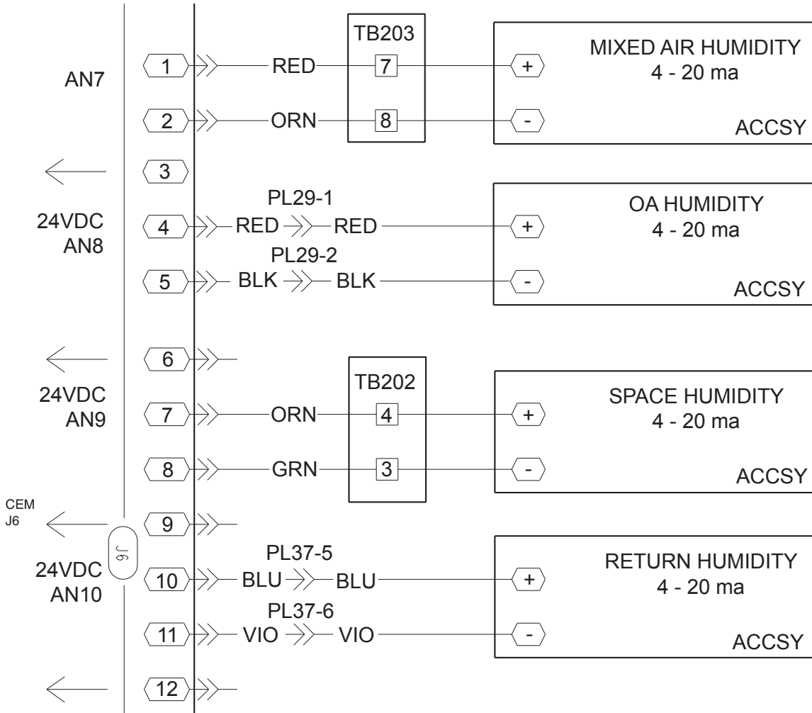
Fig. 78 — Space and Return Air Humidity Sensor Wiring
