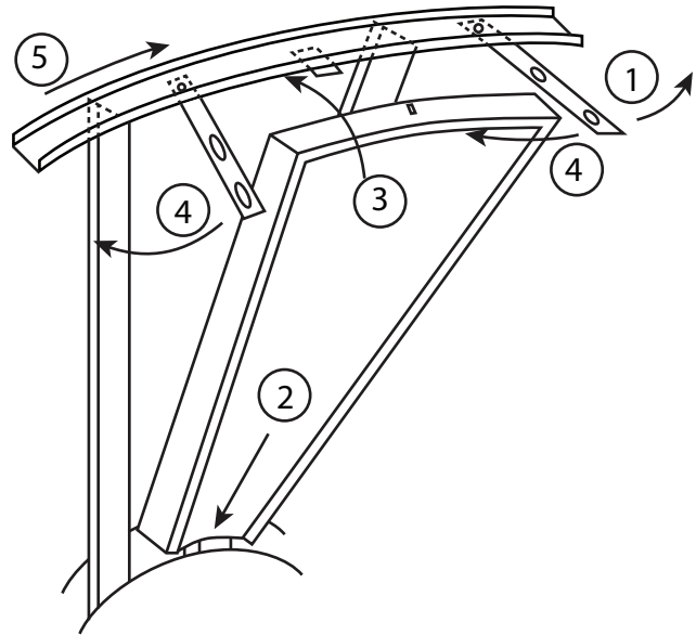
Fig. 52 — Segment Installation
