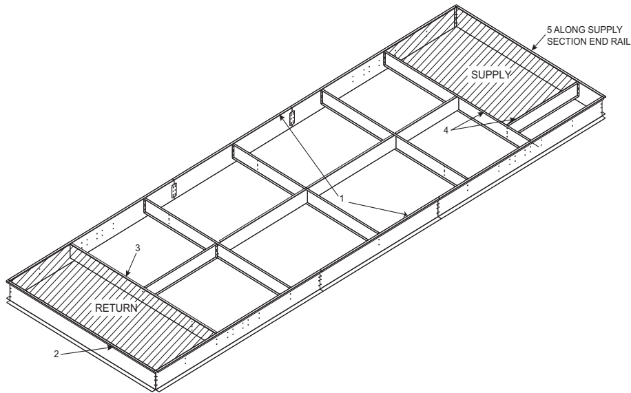
Fig. 23 — Gasket Location on Roof Curb
