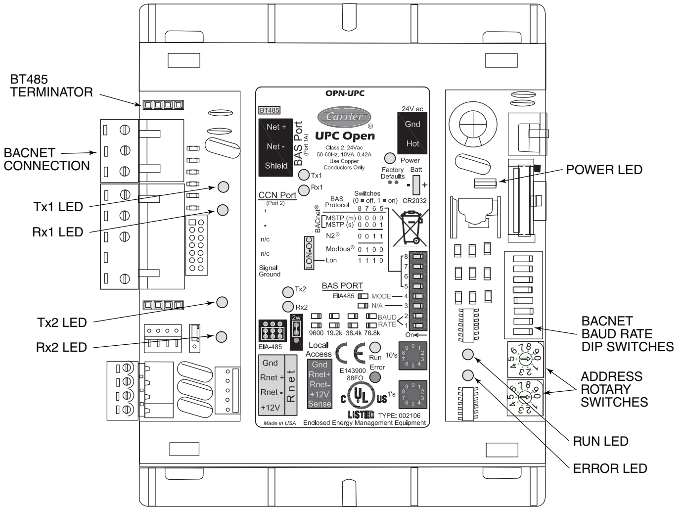
Fig. 84 — UPC Open Controller
