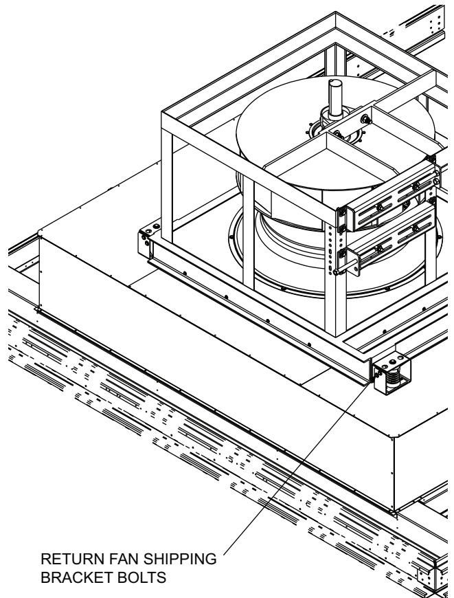
Fig. 50 — Return Fan Shipping Bracket Bolts
