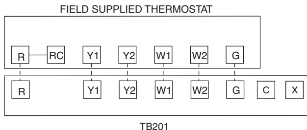
Fig. 70 — Field Control Thermostat Wiring
