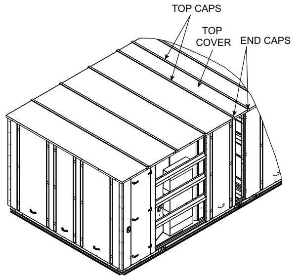
Fig. 66 — Main Unit and Return Section Top Cover Assemblies
