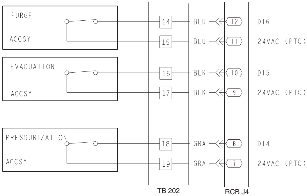
Fig. 82 — Purge, Evacuation, and Pressurization Wiring
