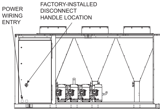
Fig. 45 — Factory-Installed Disconnect Location (End of Unit Shown)
