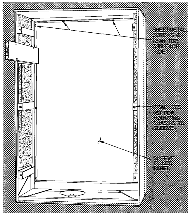
→ Fig. 1 — Wall Sleeve and Filler Panel
