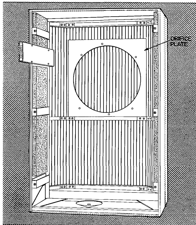
→ Fig. 2 — Deluxe Architectural Grille Installed
