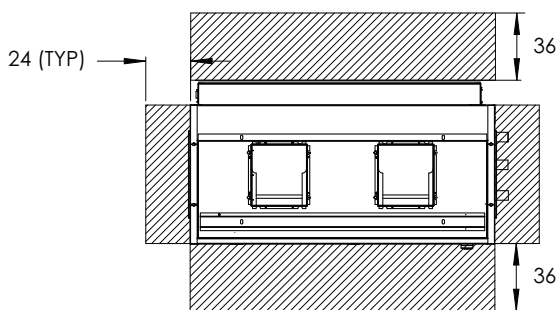
Fig. 11 — Unit Clearances
