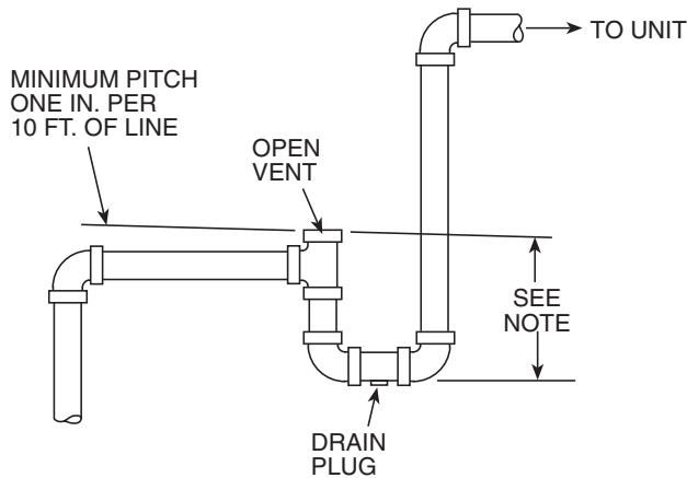
Fig. 15 — External Trap Condensate Drain
