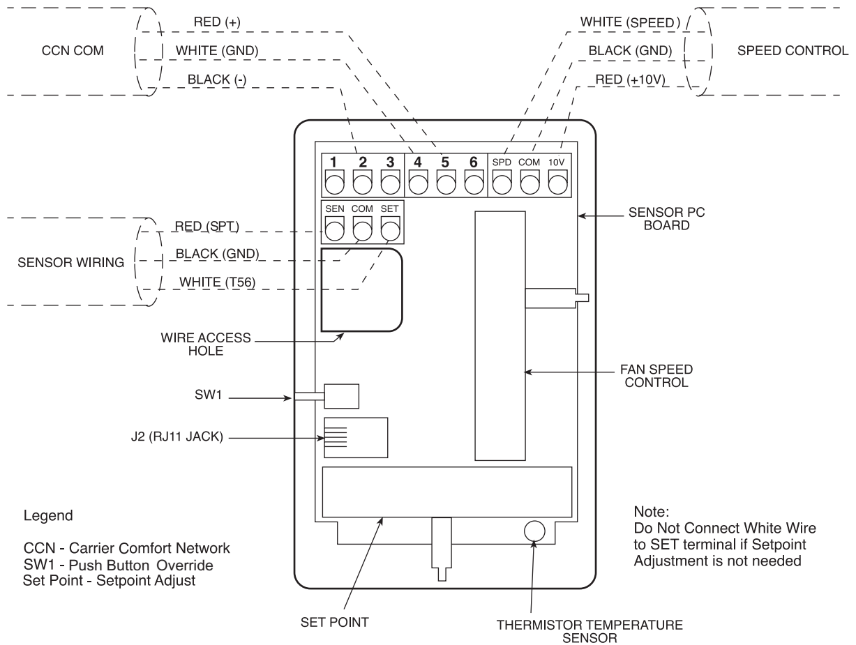
Figure 2 T-57 Space Temperature Sensor Wiring
