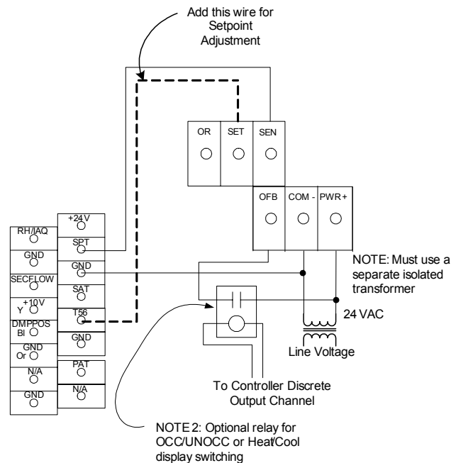
Figure 2 T-59 Space Temperature Sensor - Wiring
