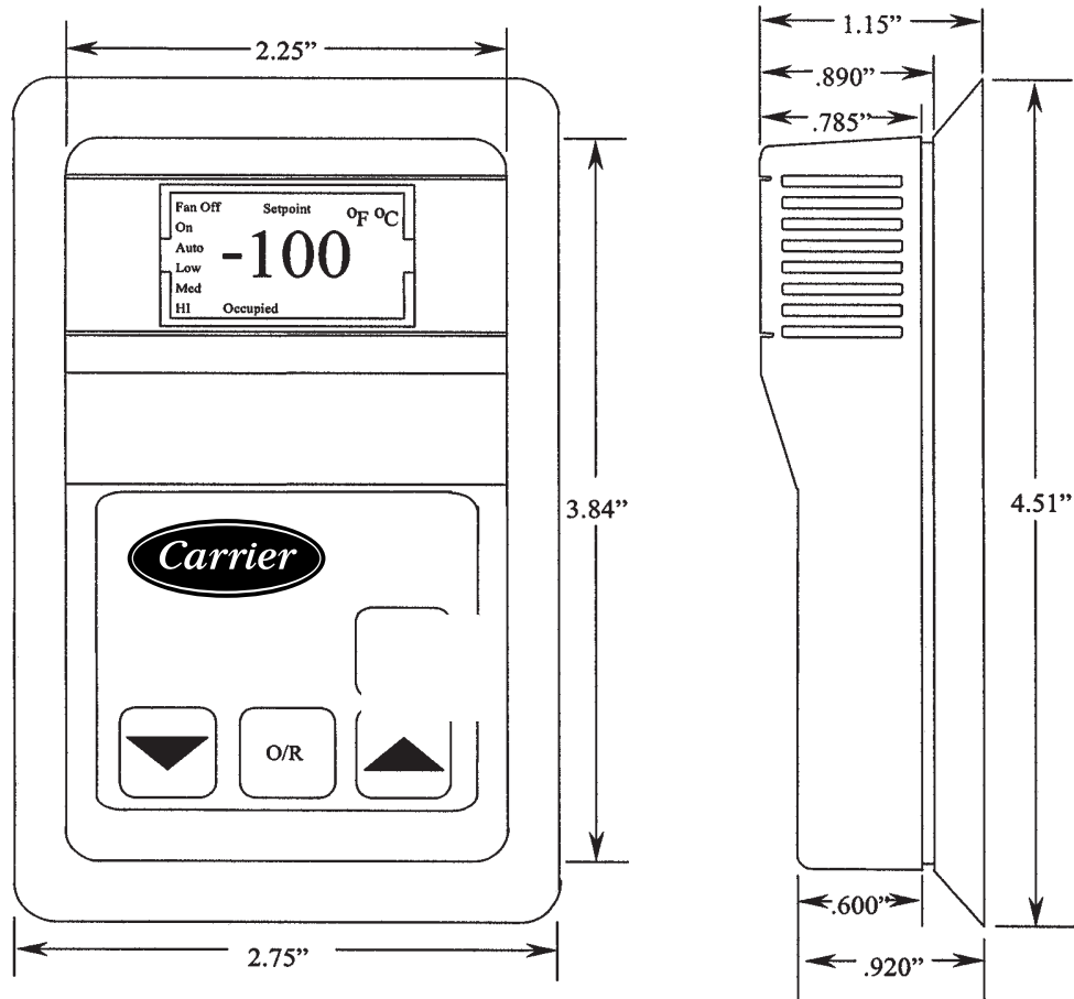
Figure 1 T-59 Space Temperature Sensor
