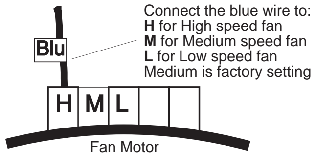
Figure 19: PSC Motor Speed Selection
