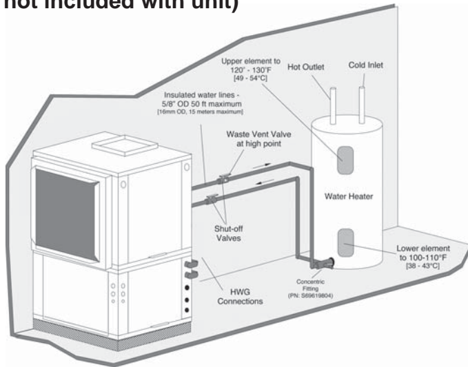
Figure 16: Alternate HWG Piping with concentric/coaxial fitting (part #S69619804 not included with unit)
