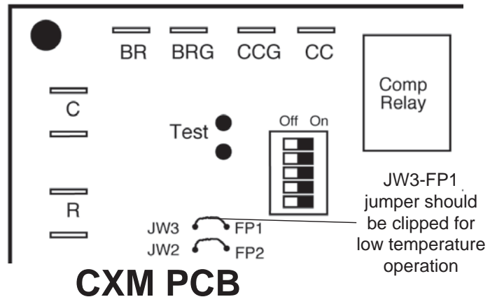
Figure 22: FP1 Limit Setting
