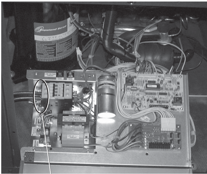
Figure 17: GT-PX/GT-PG Single Phase Line Voltage Field Wiring
