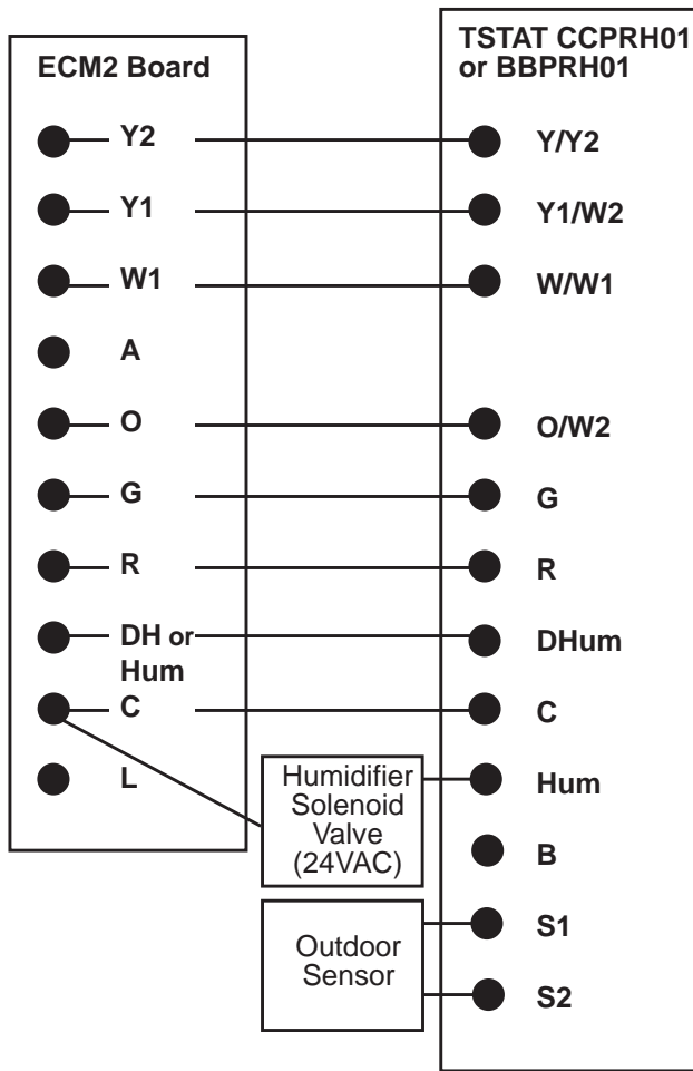
Figure 27: Thermidistat (Carrier TSTATCCPRH01) (Bryant TSTATBBPRH01)
