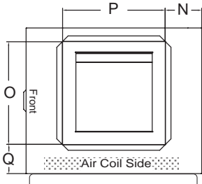
Top View-Right Return
