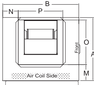
Top View-Left Return
