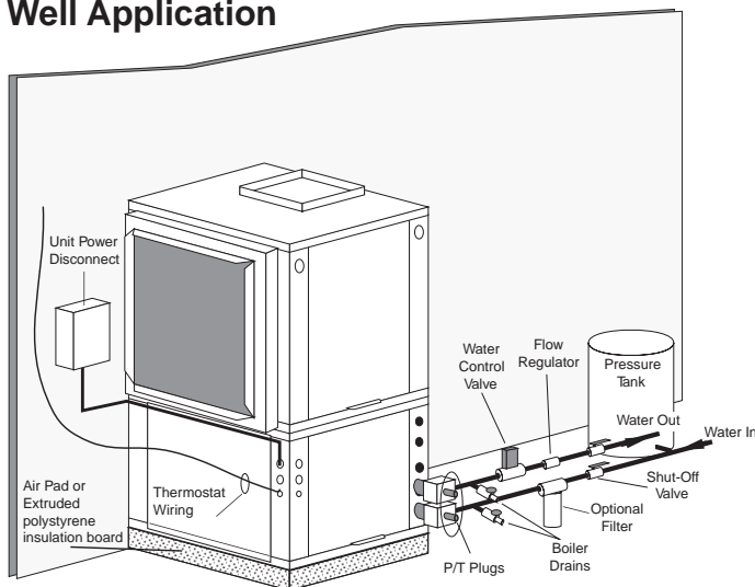
Figure 13: Typical Open Loop/Well Application
