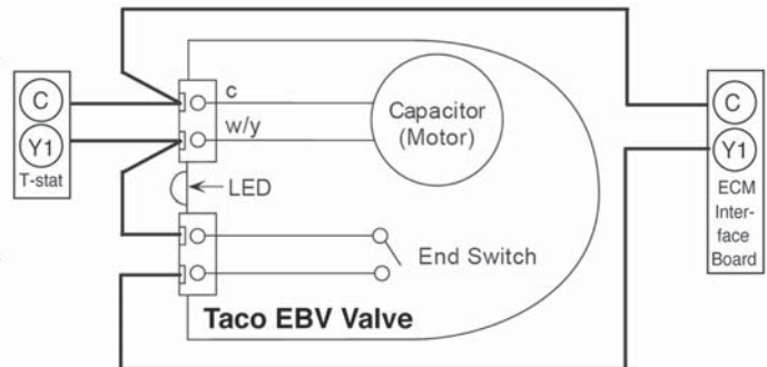
Figure 25: Taco ESP Valve Wiring
