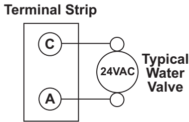
Figure 23: Accessory Wiring
