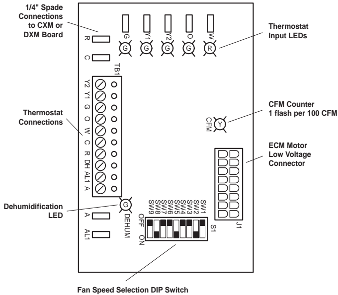
Figure 29a: ECM Version II Interface Layout
