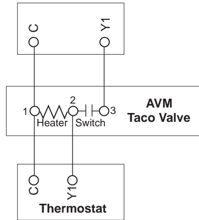
Figure 24: AVM Valve Wiring
