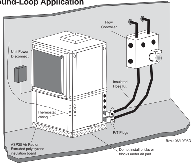
Figure 12: Typical Ground-Loop Application
