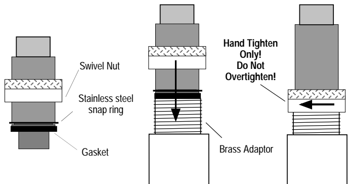
Figure 11: Water Connections
