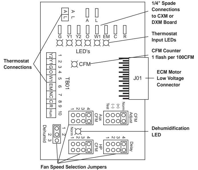
Figure 29b: ECM Version I Interface Layout
