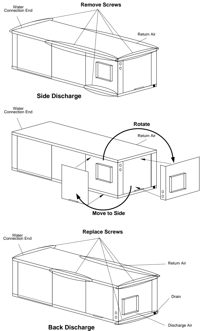
Figure 5: Right Return Side to Back
