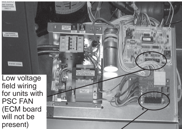
Figure 20: GT-PX/GT-PG Low Voltage Field Wiring
