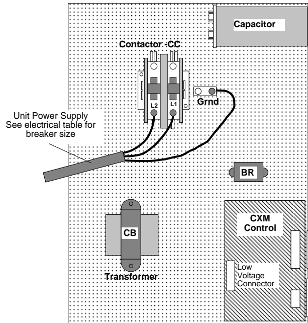
Figure 18: GT-G Single Phase Line Voltage Field Wiring
