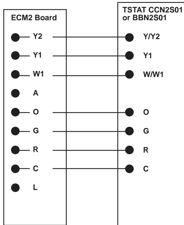
Figure 28: Non-Programmable Thermostat (Carrier TSTATCCN2S01) (Bryant TSTATBBN2S01)
