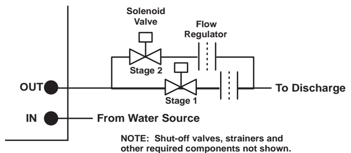
Figure 26: Two-Stage Piping
