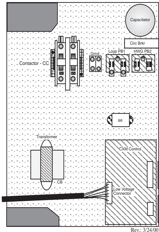
Figure 21: GT-G Low Voltage Field Wiring
