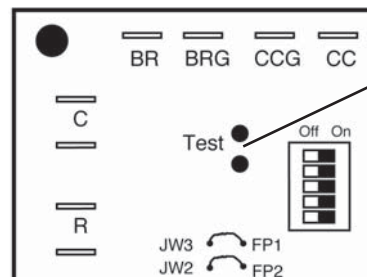
Figure 30: Test Mode Pins
