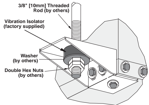
Figure 1: Hanger Bracket
