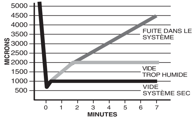
Figure 17 – Courbe de vide
