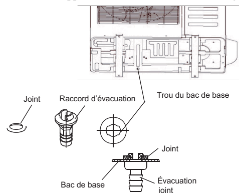
Figure 13 – Raccord de flexible d'évacuation
