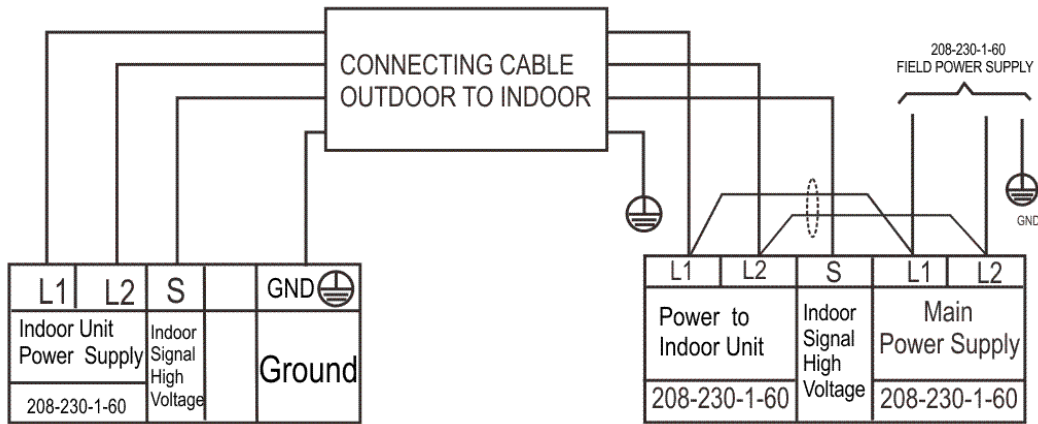
Figure 23 – Schémas de raccordement – capacités 18 to 24
