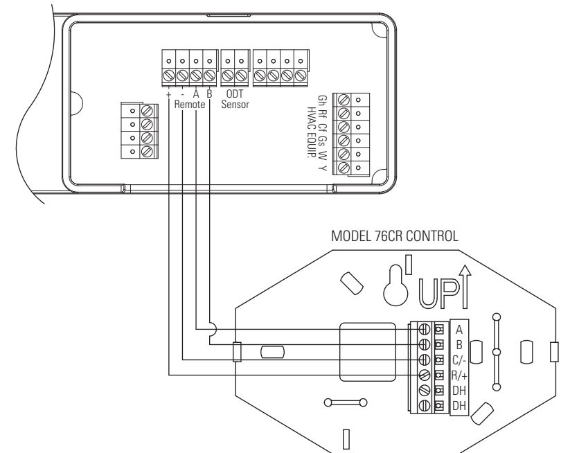
FIGURE 7 – Model 76CR Remote Control Wiring
