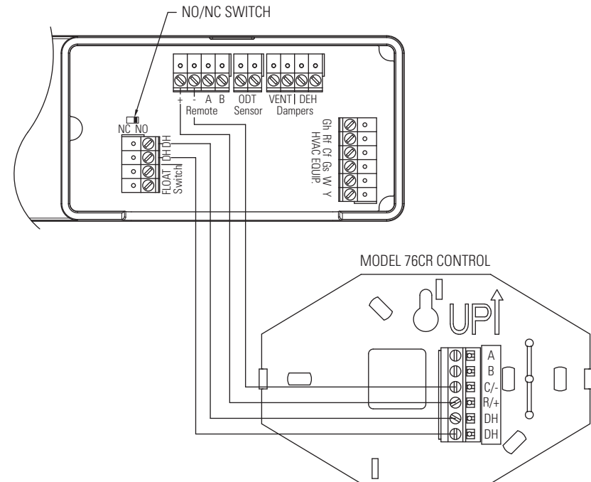
FIGURE 5 – Model 76CR External Control Wiring
