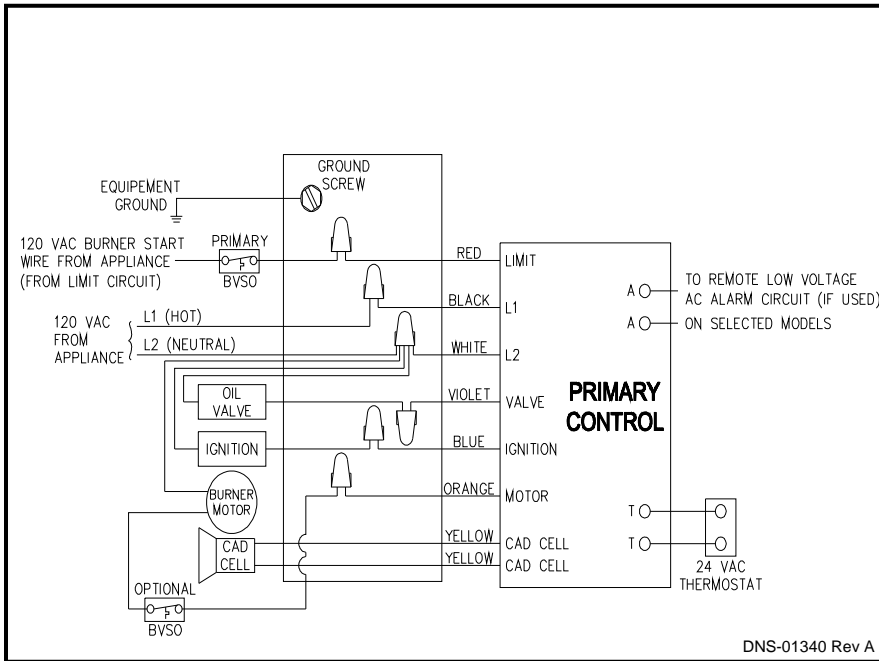
Beckett Burner
