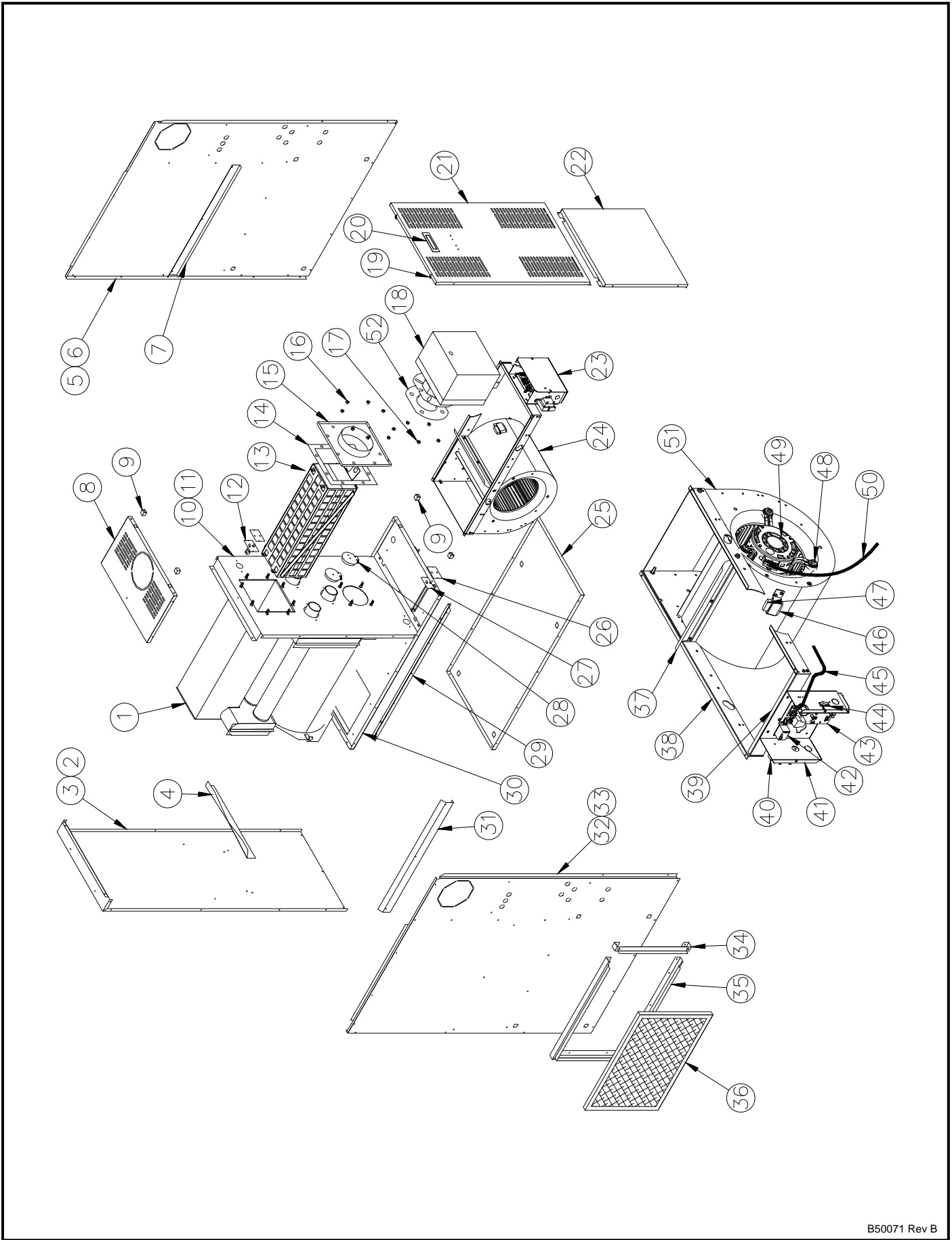
Figure 17 : Parts list - CBMAAR060120
