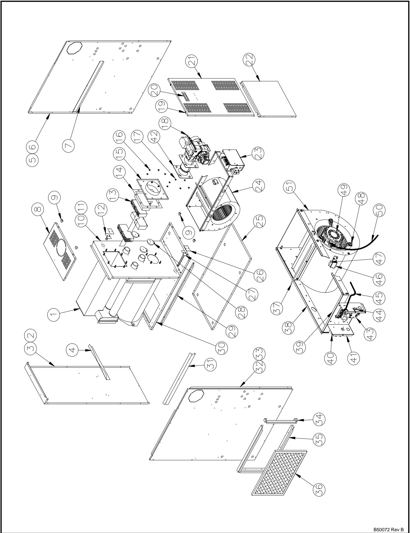
Figure 15 : Parts list - CBMAA060120
