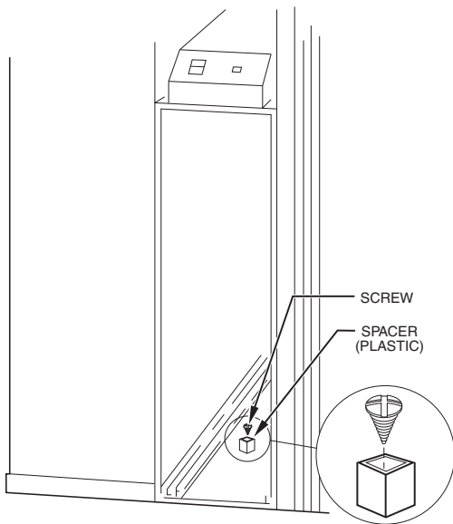
Fig. 8 - Plastic Positioning Spacer
