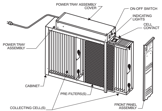
Fig. 1 - Unit Assembly
