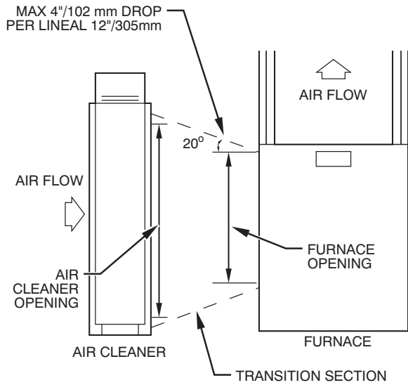
Fig. 5 - Transition to Unit
