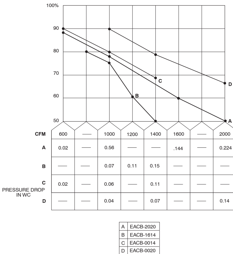
Fig. 2 - Efficiency and Pressure Drop Performance
