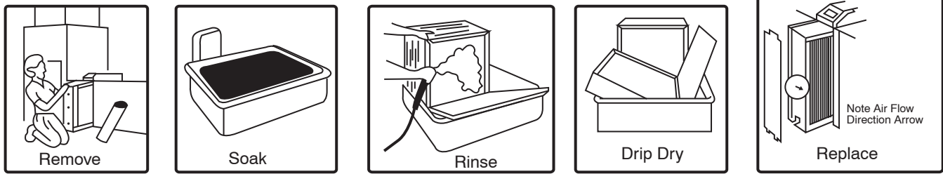
Fig. 11 - Typical Call and Prefilter Cleaning
