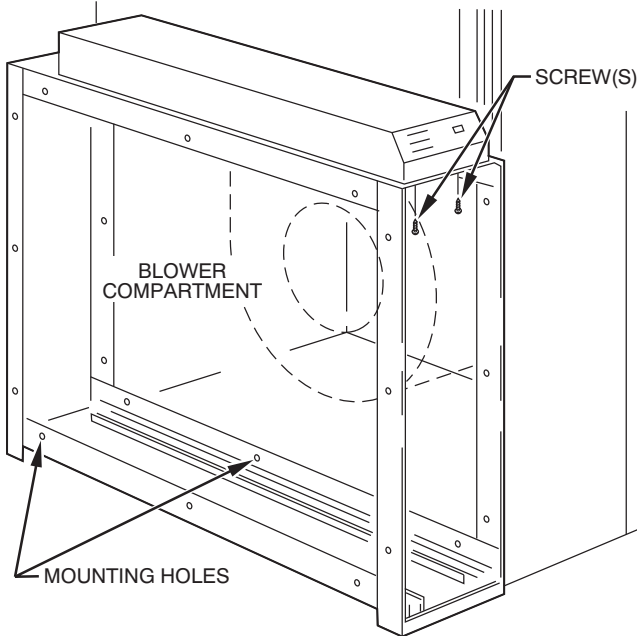
Fig. 9 - Mounting Hole Location
