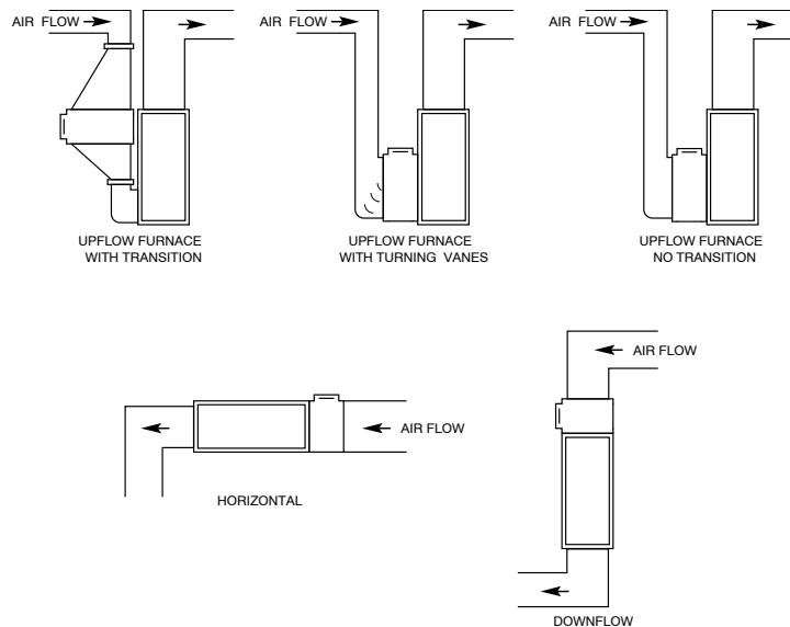
Fig. 7 - Typical Installations
