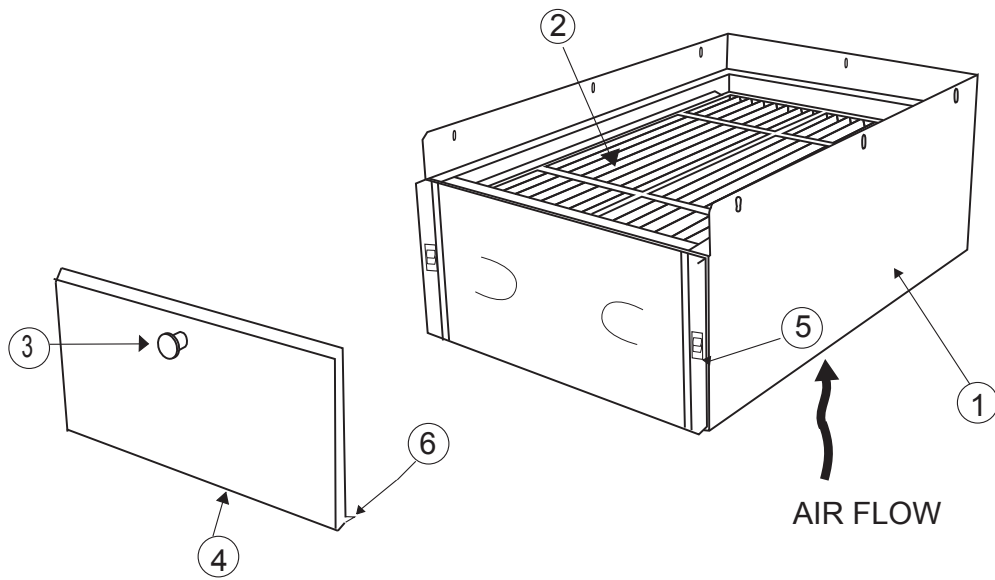
Fig. 2 - FNCCAB Major Components
