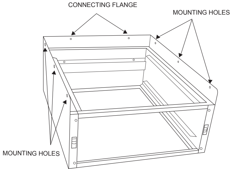
Fig. 5 - Mounting Holes and Mounting Flange
