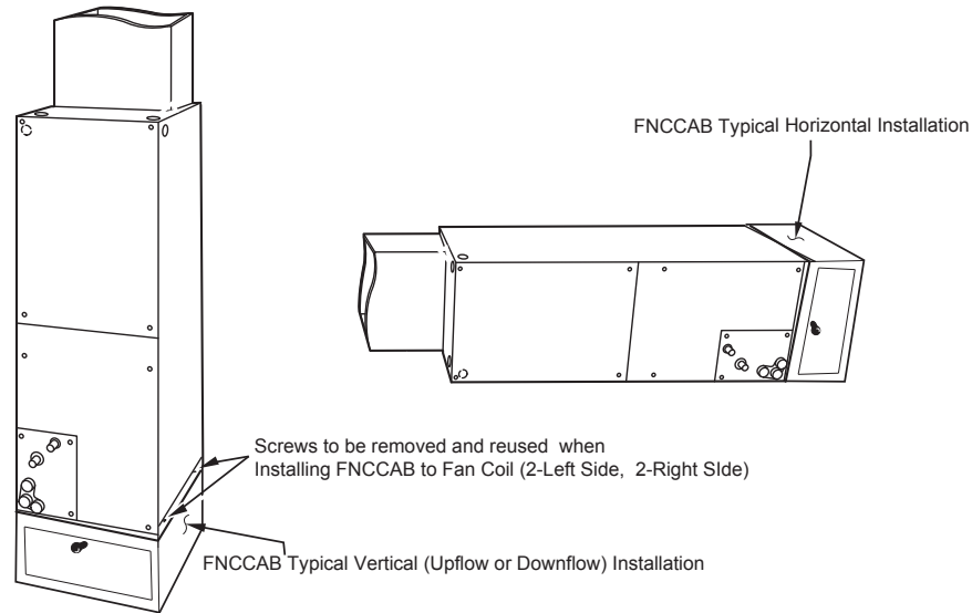
Fig. 4 - Typical Installation
