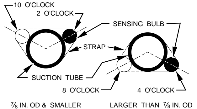
Fig. 4—Position of Sensing Bulb
