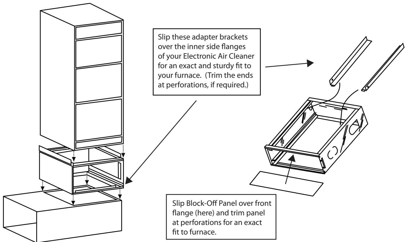
Fig. 1 - Block-Off Panel Assembly
