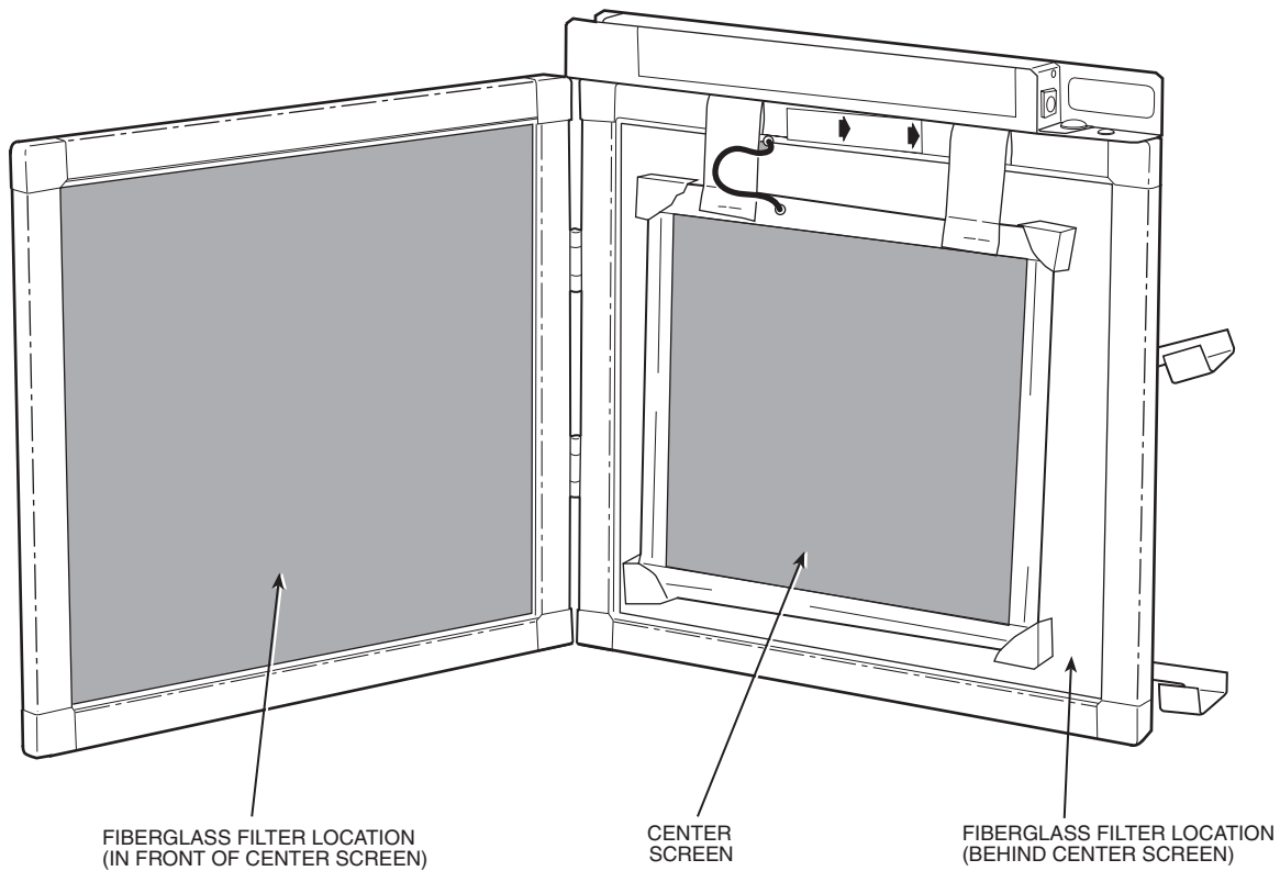
Fig. 2 — Filter Replacement
