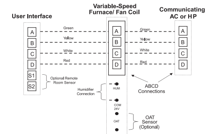
Fig. 2 - Four-Wire Connection Diagram
