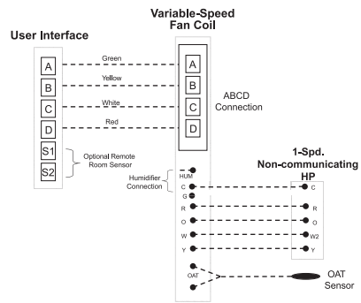
Fig. 4 - Connection Diagram for FE Fan Coil with Non-Communicating 1-stage HP
