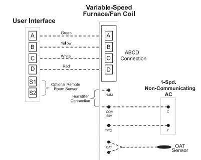
Fig. 2 - Four-Wire Connection Diagram
