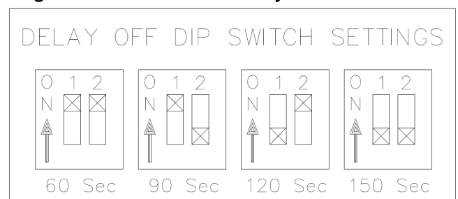
Figure 8 – Blower “OFF” delay - Board #ST9103A
